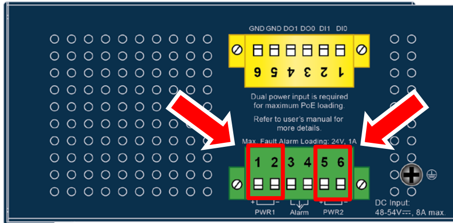
Figure 2-1-5: Upper Panel
