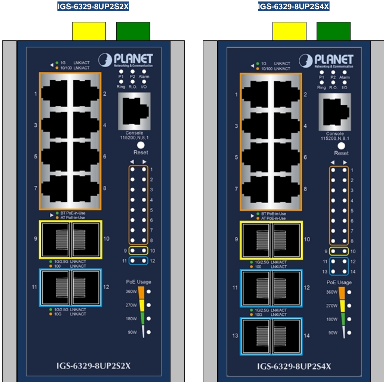
Figure 2-1-1 IGS-6329-8UP2S2X and IGS-6329-8UP2S4X Switch Front Panel
