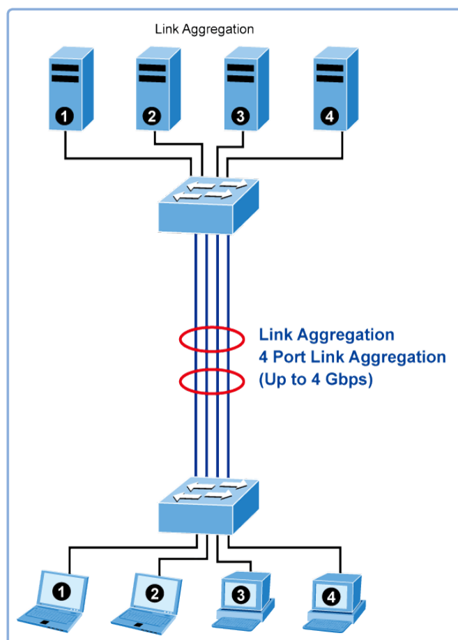
Figure 4-3-2-1: Link Aggregation
