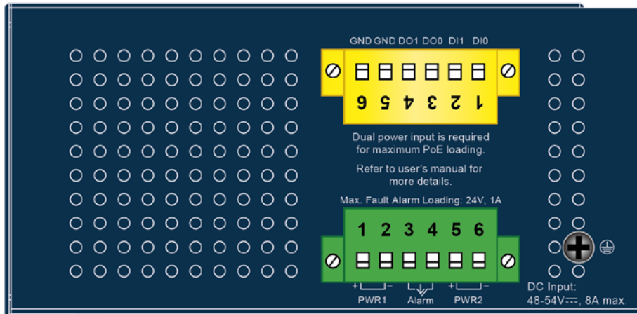
Figure 2-1-6 Wiring the DI and DO of switch
