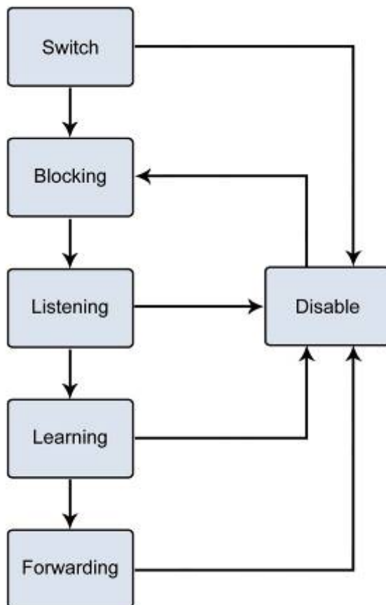
Figure 4-3-10-1-1: STP Port State Transitions
