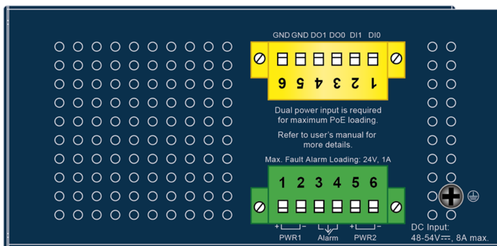
Figure 2-1-4: Upper Panel of IGS-6329-Series
