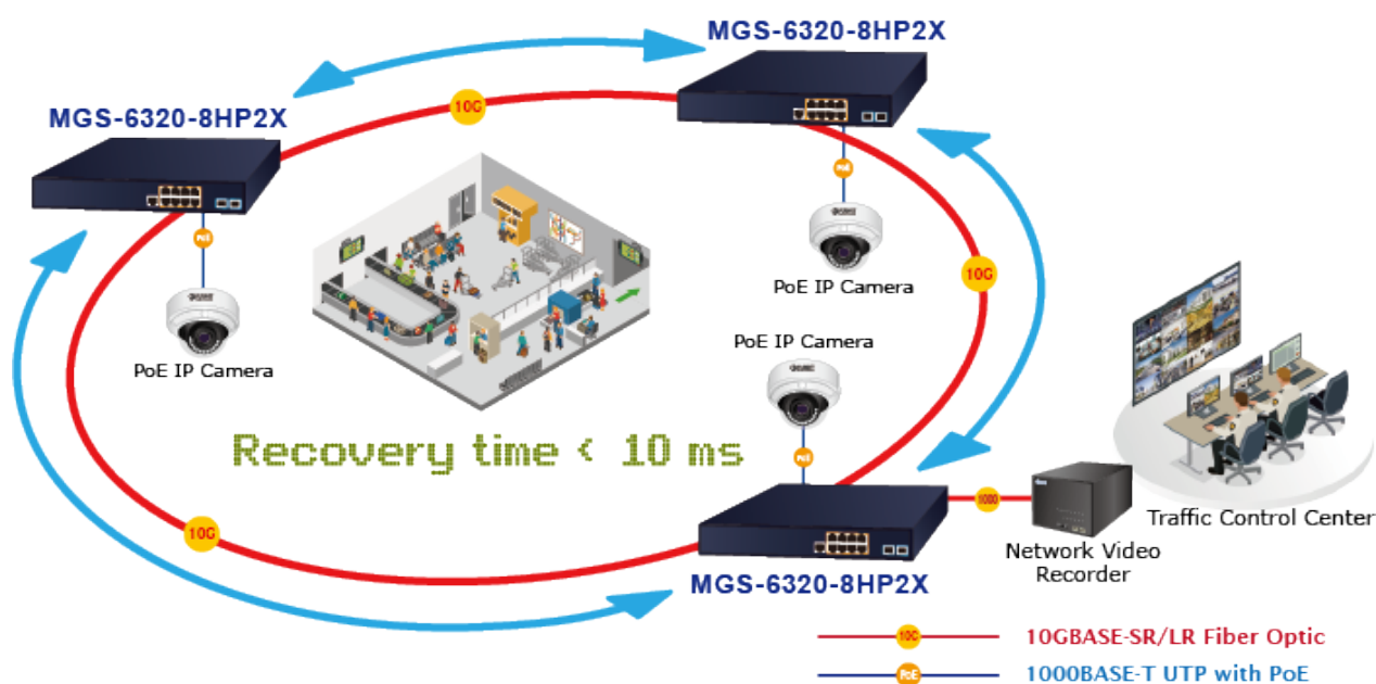
Figure 4-8-6-1: Ring Example Diagram
