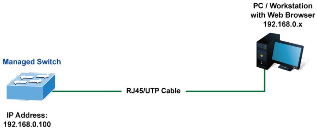
Figure 3-3: Web Management
