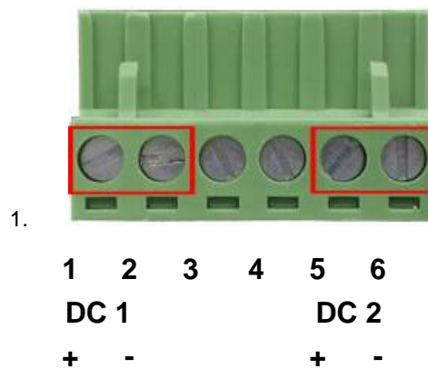
Figure 2-1-12 6-pin Terminal Block Power Wiring Input
