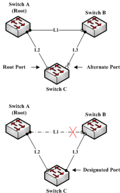
Figure 1.4 Backbone Fast
