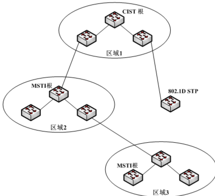
Figure 2.1 MSTP topology
