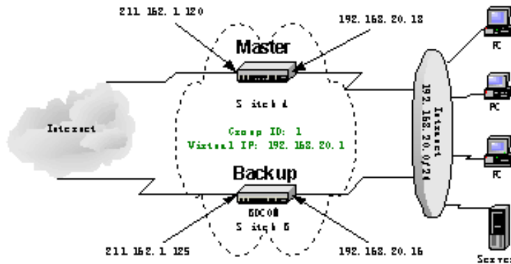
Figure1 69-1 Network topology
