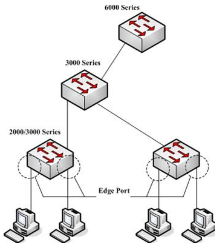
Figure 2.7 Edge port
