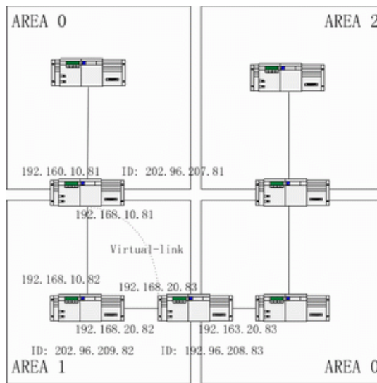
Figure 4-2 Network topology of the configuration example
