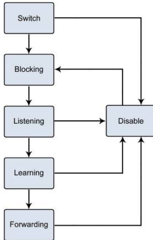
Figure 4-3-4-1: STP Port State Transitions
