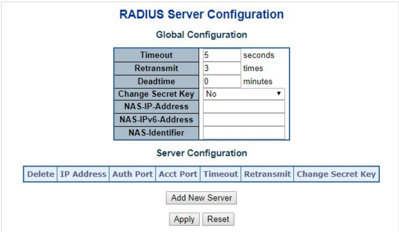
Figure 4-5-2-4: RADIUS Server Configuration Page Screenshot
