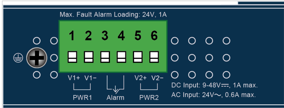
Figure 2-1: IGT-900 Series Upper Panel
