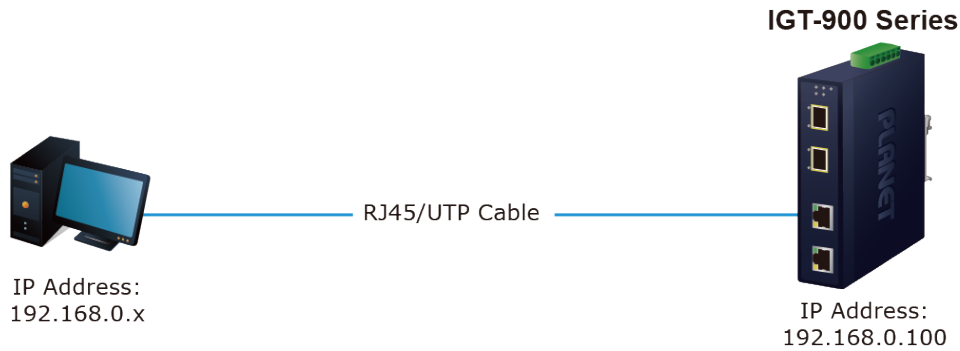
Figure 3-3: Web Management
