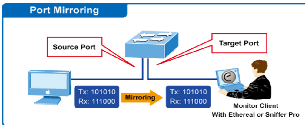
Figure 4-3-1-5: Port Mirror Application
