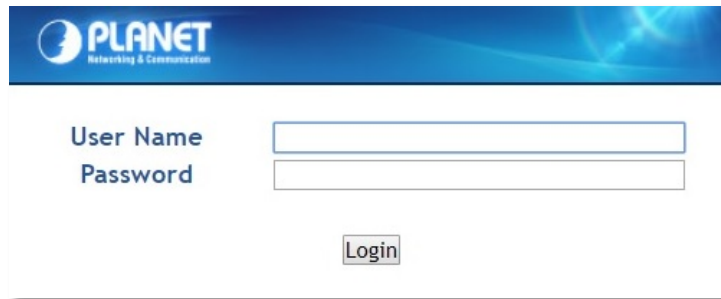
Figure 4-1-2: Login Screen
