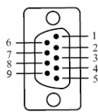
DB9M (Male/needle)
