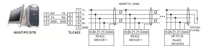
Figure 2: Master/Slave multi-drop configuration
