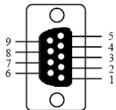
DB9F (Female/hole)
