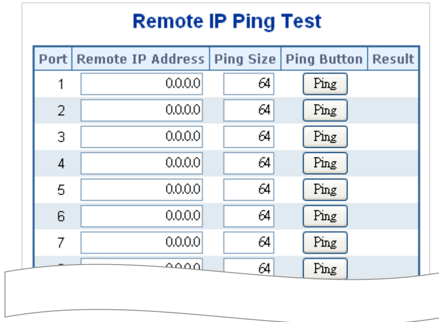
Figure 4-8-2-3: Remote IP Ping Test Page Screenshot
