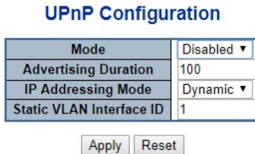
Figure 4-2-11: UPnP Configuration Page Screenshot
