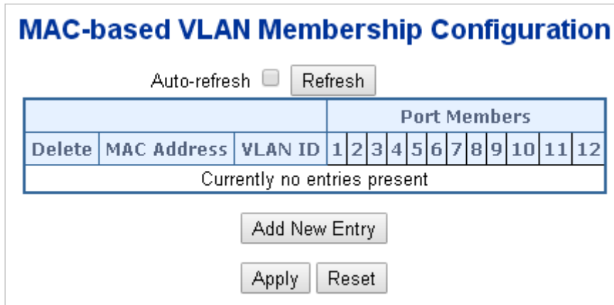
Figure 4-3-3-16: MAC-based VLAN Membership Configuration Page Screenshot
