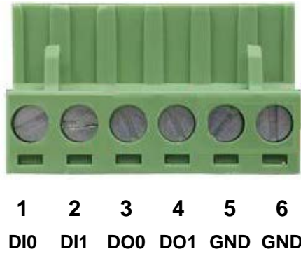
Figure 2-14: 6-pin Terminal Block for DI and DO Wiring Input
