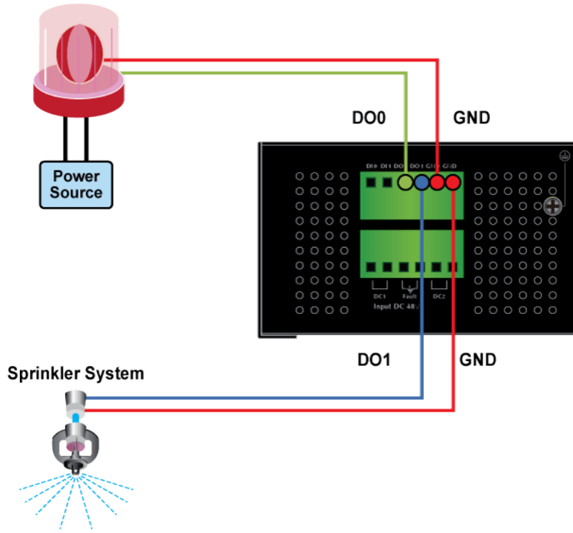
Figure 2-10 Wires DO0 and DO1 to Open Detector
