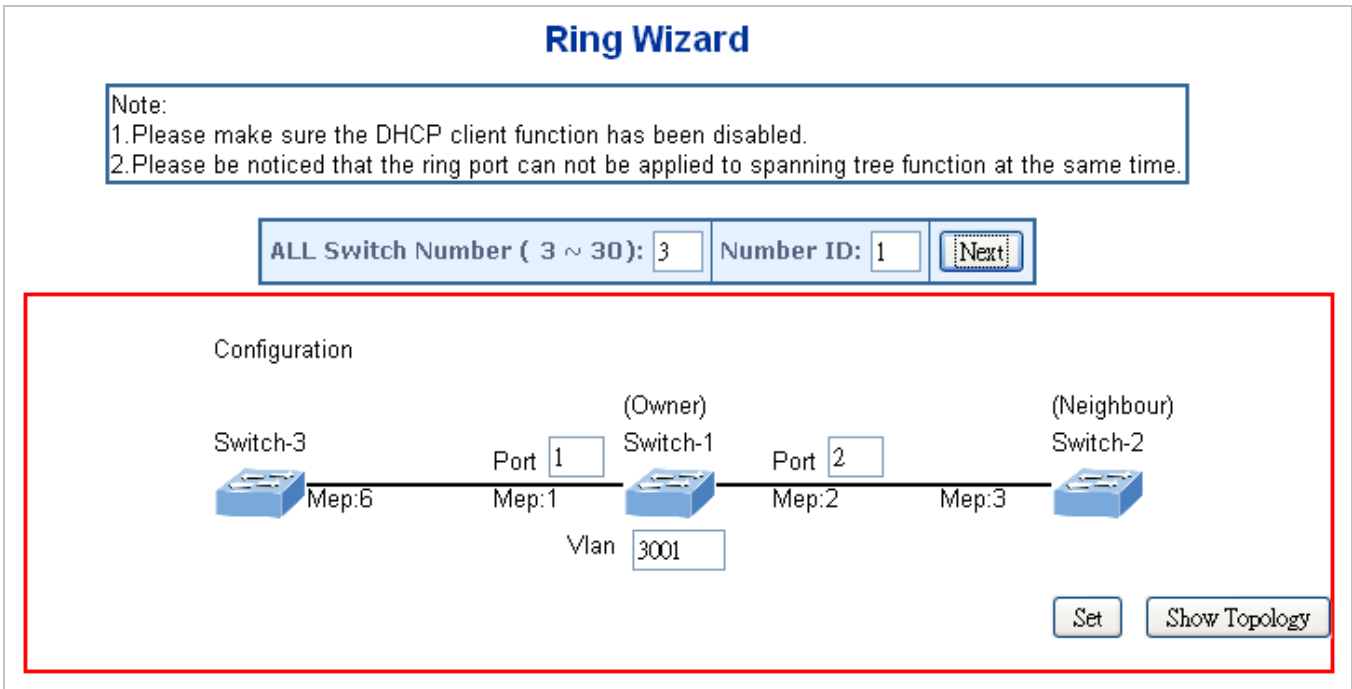
Figure 4-7-1-5: Ring Wizard page screenshot
