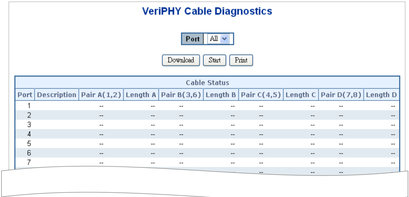
Figure 4-9-2-4 VeriPHY Cable Diagnostics Page Screenshot
