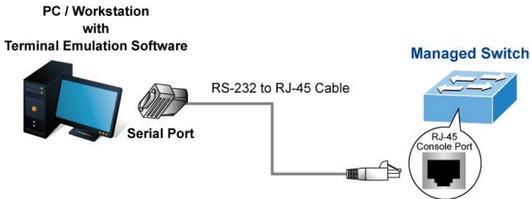
Figure 3-1 Out-of-Band Management Configuration Environment
