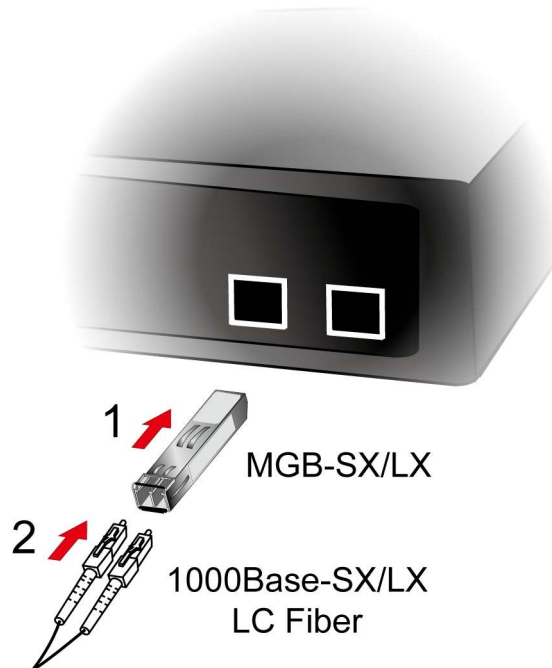
Figure 2-4 Plug in the SFP transceiver
