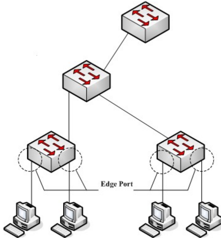
Figure 2.7 Edge port
