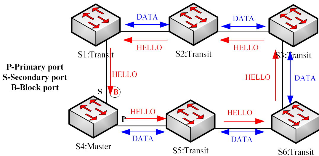
Figure 3: Polling
