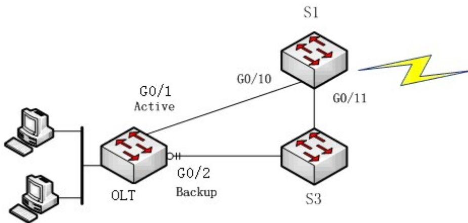
Figure 1: FlexLinkLite-enabled network
